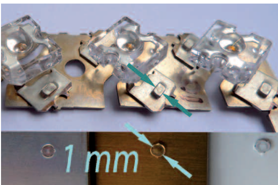
Micro clinch
