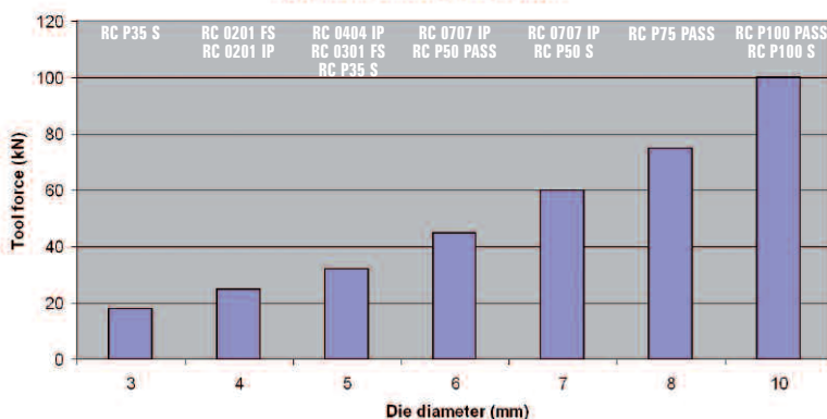
Tool force versus die diameter
