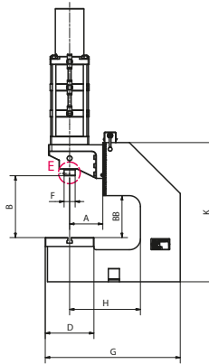
XL-DA Type
